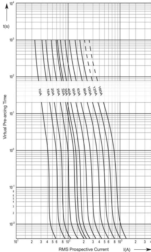
Time-Current Characteristics
