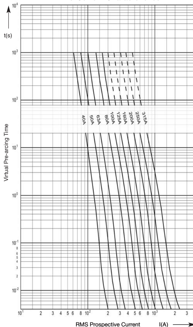
Time-Current Characteristics
