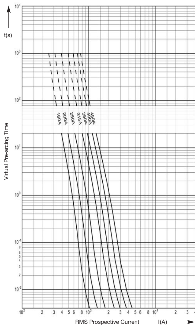
Time-Current Characteristics
